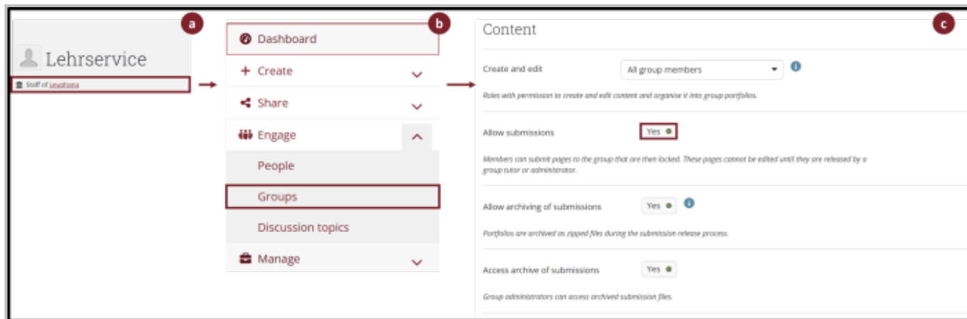
Fig. 2: Allow submissions
