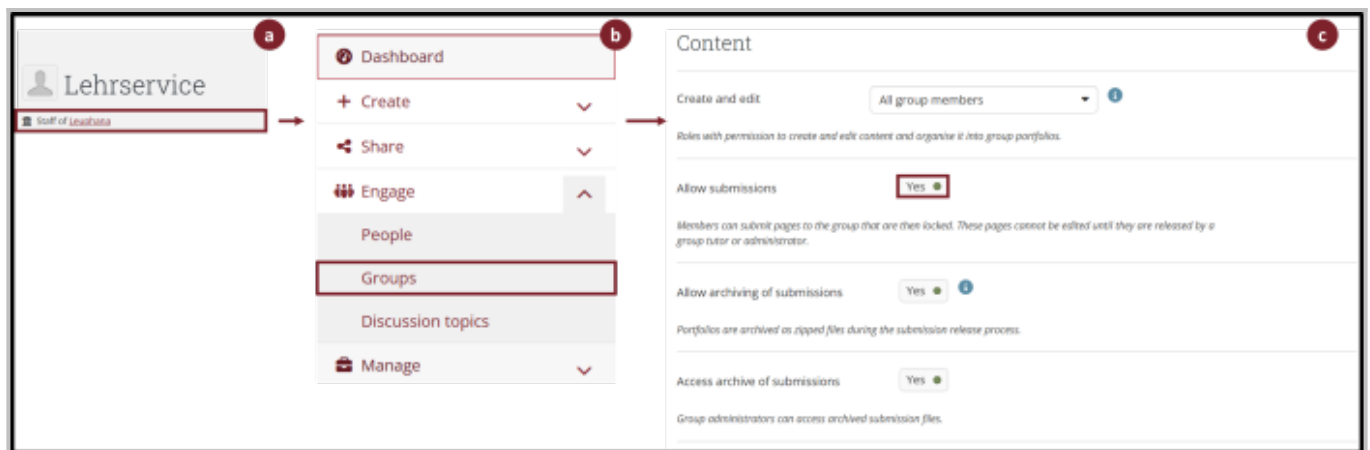
Fig. 2: Allow submissions
