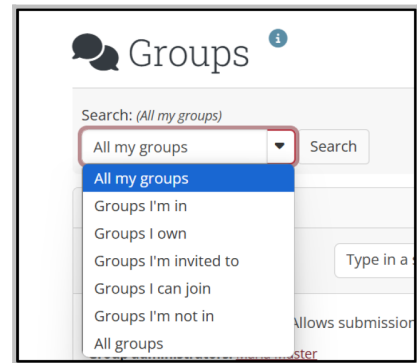
Fig. 4: Group search
