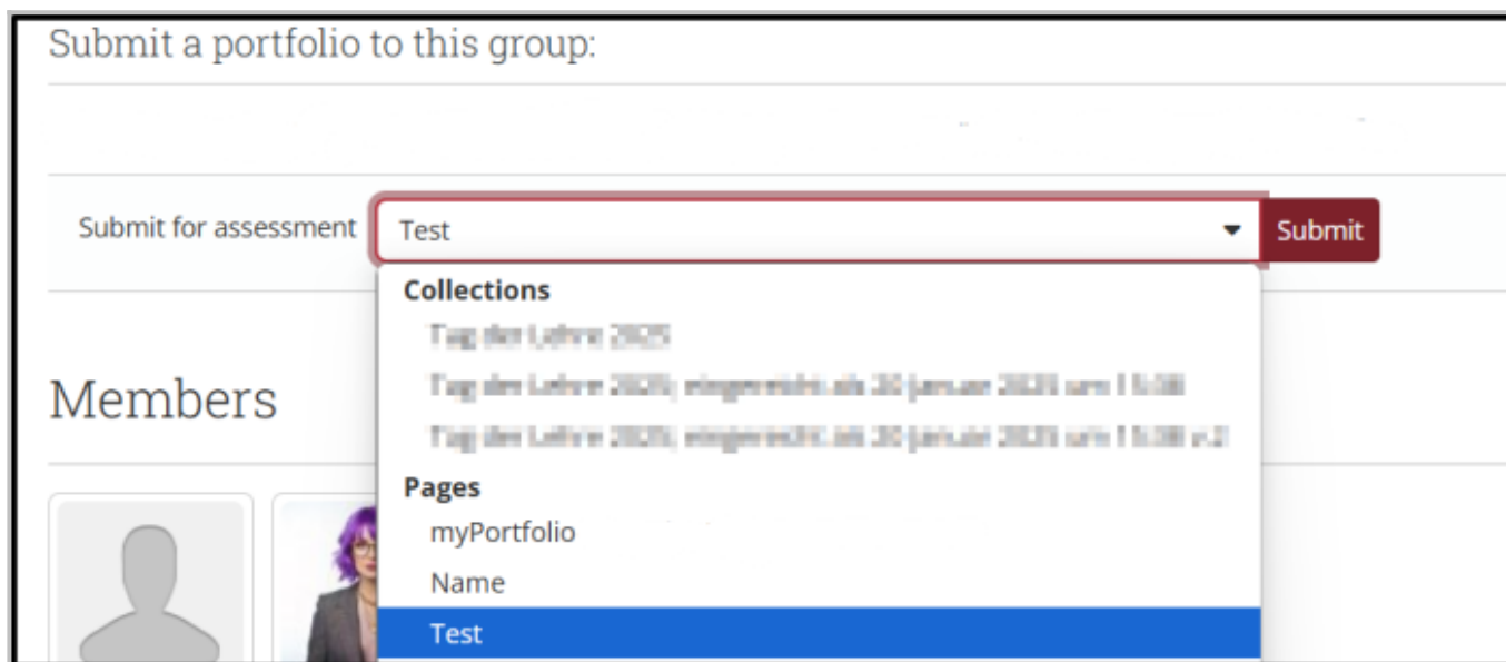
Abb. 2: Allow submissions
