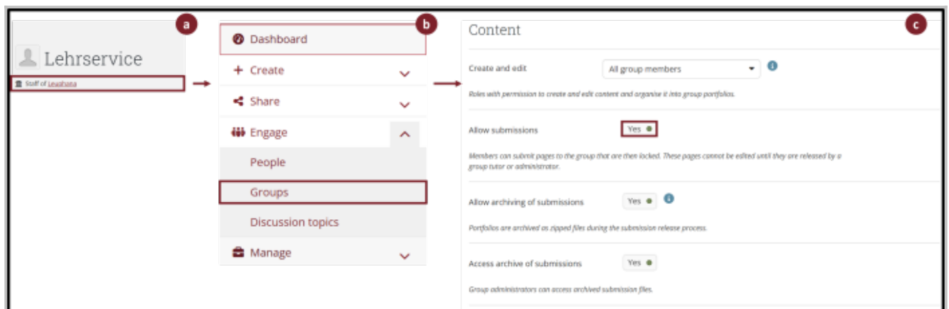
Abb. 1: Allow submissions
