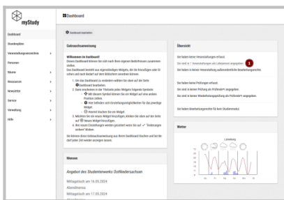
Fig. 2: Dashboard
